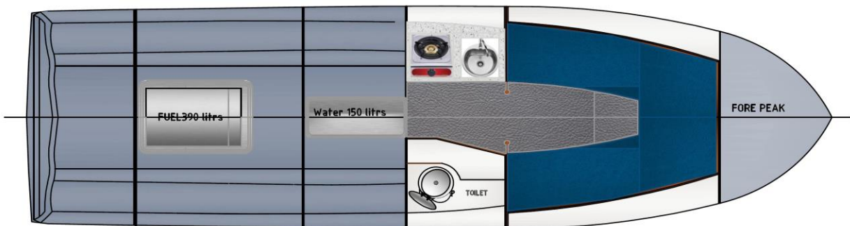
BELOW DECK PLAN
