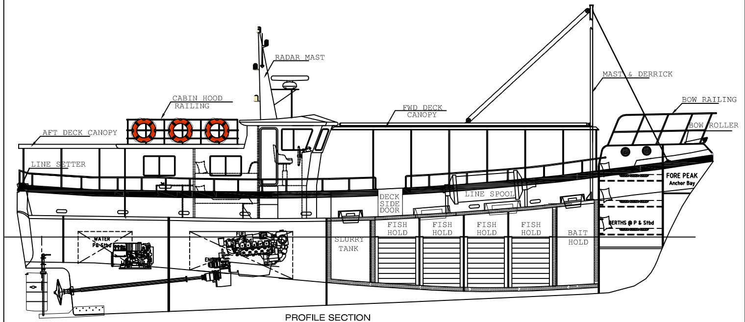
PROFILE SECTION
