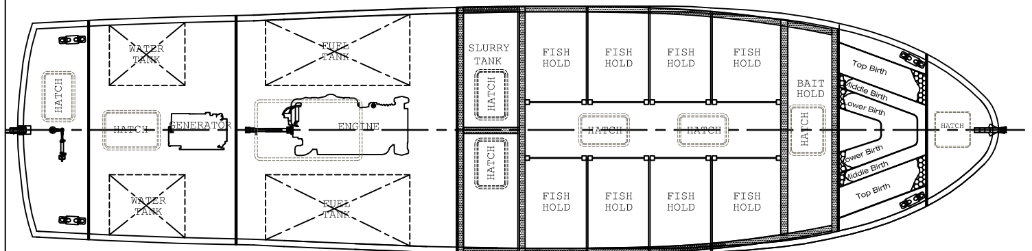
BELOW DECK PLAN
