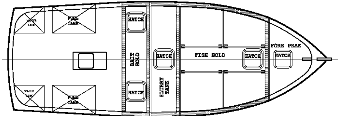
BELOW DECK PLAN
