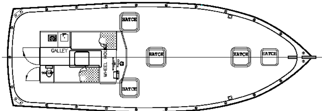
DECK PLAN
