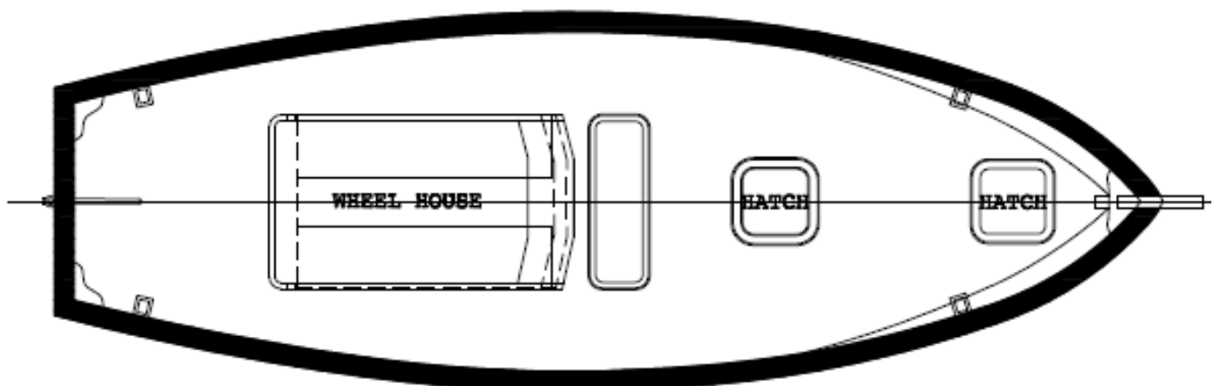
DECK PLAN
